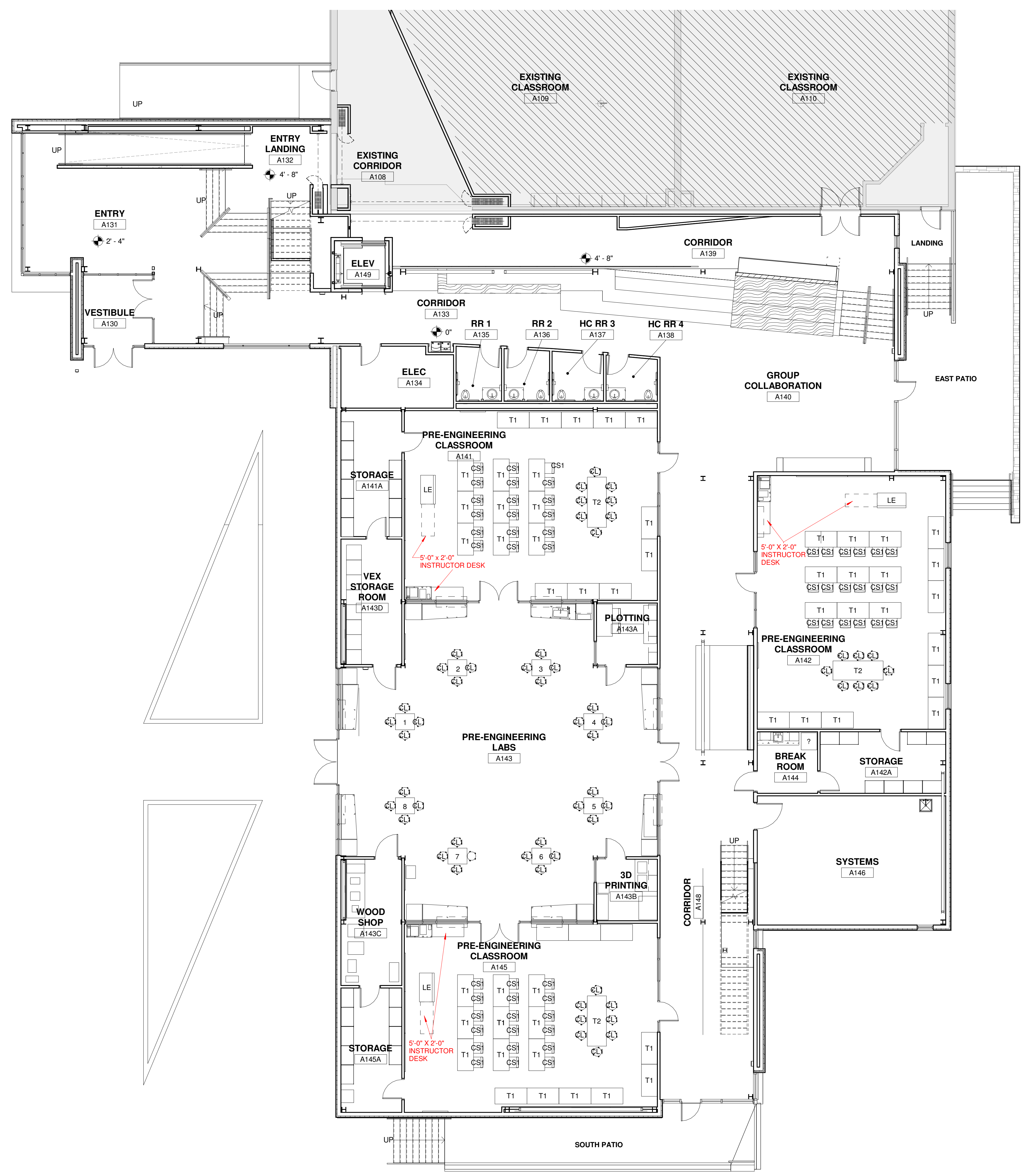
A1 FIRST FLOOR FURNITURE PLAN Scale: 1/8" = 1'-0"
